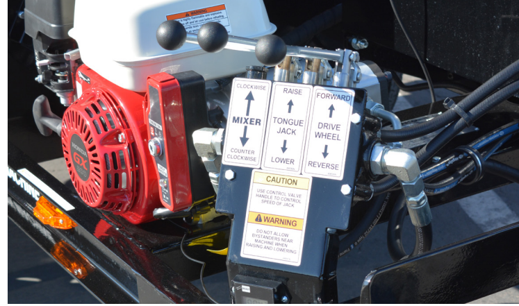
E-Z Operating Controls
