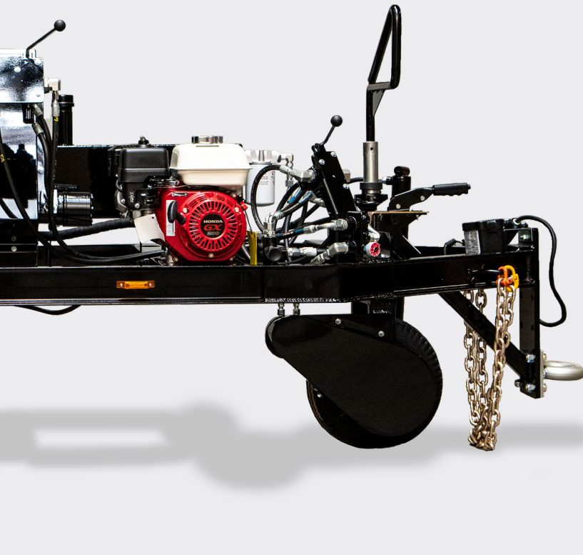
Power Drive Wheel and E-Z Steer Assembly
